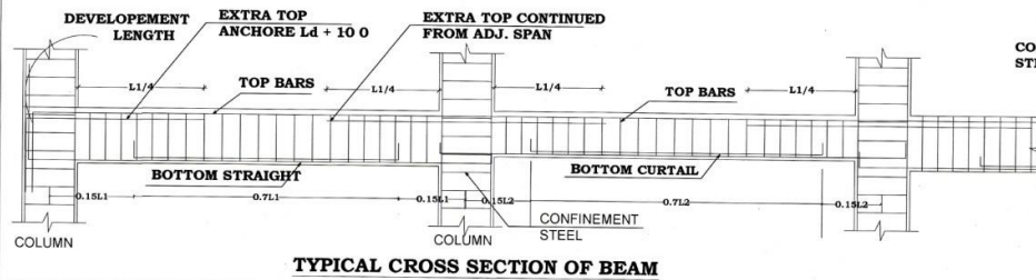
TYPICAL CROSS SECTION OF BEAM
