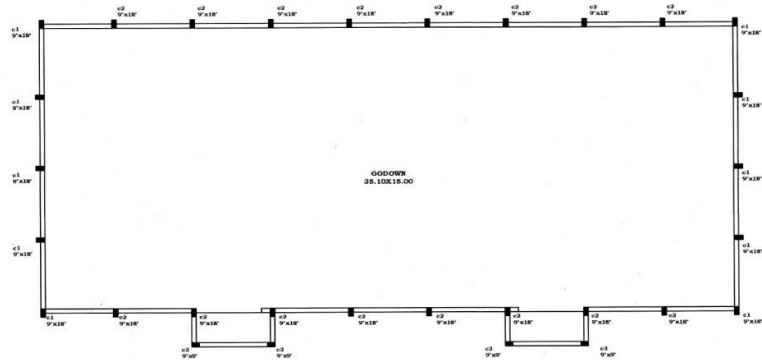
SCHEDULE OF FOOTING AND COLUMNS (up to g.f. slab only)
