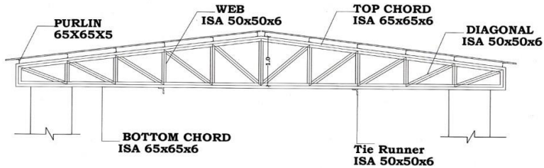
ELEVATIONAL DETAILS OF ROOF TRUSS
