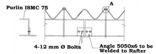
DETAILS OF PURLIN
