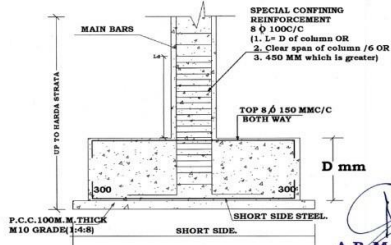
SECTION OF FOOTING
