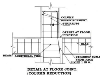
DETAIL AT FLOOR JOINT. (COLUMN REDUCTION)
