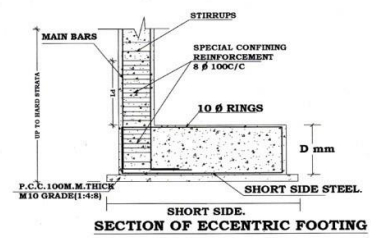
SECTION OF ECCENTRIC FOOTING
